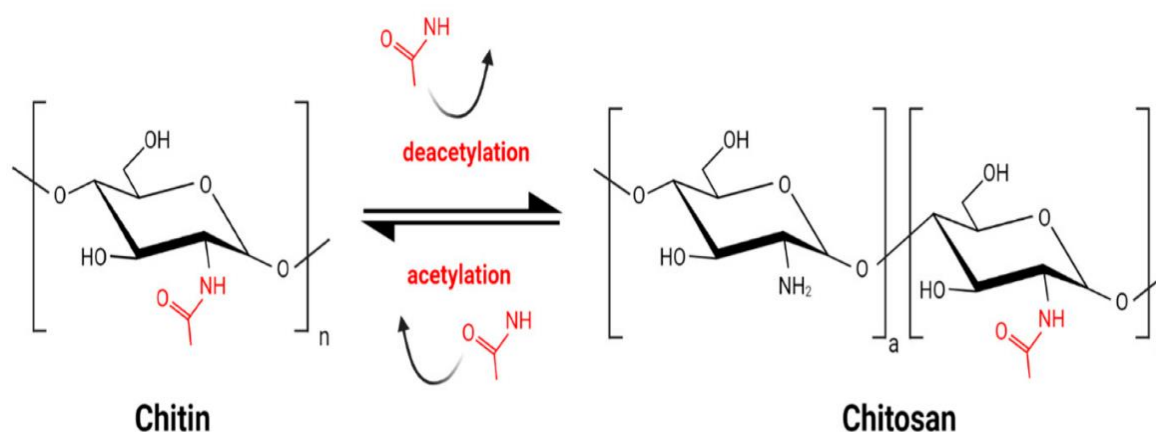
Scheme 1. Deacetylation of chitin to produce chitosan
