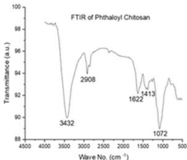
Fig. 4. FTIR spectra of phthaloyl chitosan
