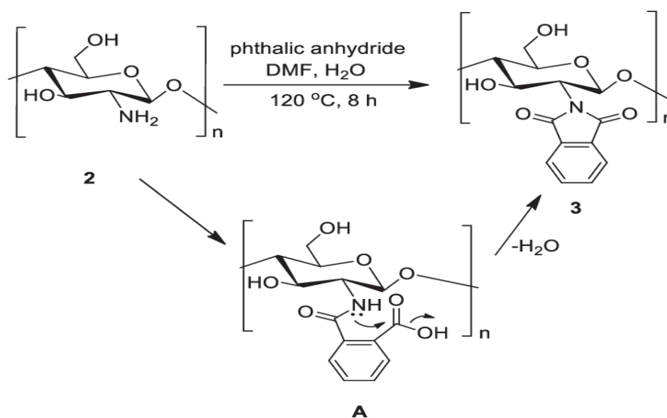
Scheme 2. Phthaloylation of chitosan by phthalic anhydride/DMF, H 2 O
