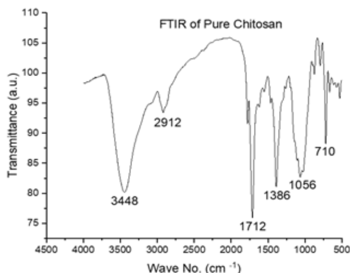
Fig. 3. FTIR spectra of pure chitosan
