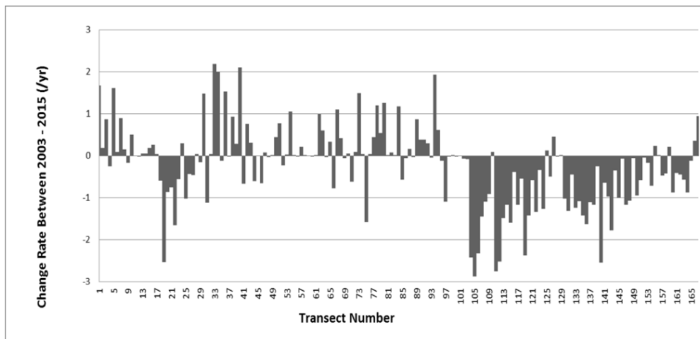
Fig. 7d. shoreline change rate between 2003-2015 (m/y)
