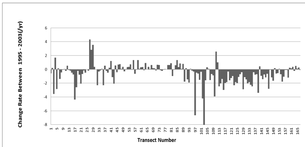
Fig. 7c. Shoreline change rate between 1995-2003 (m/y)
