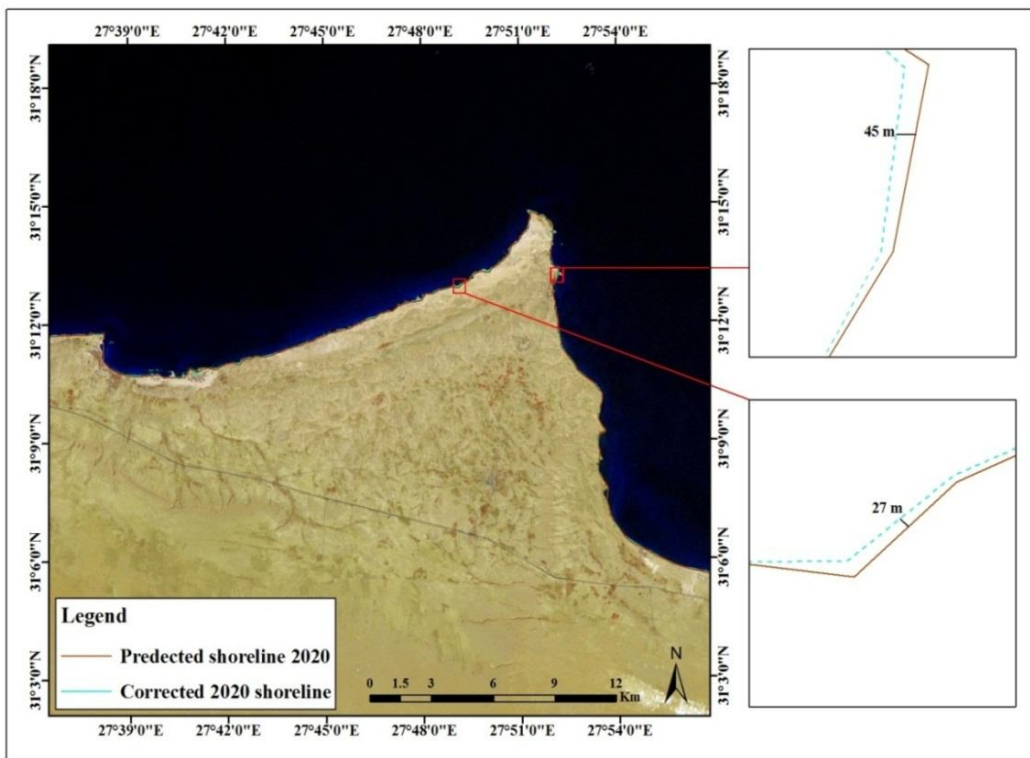
Fig. 10a. Predicted 2020 shoreline and its correction
