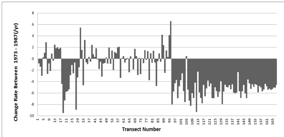
Fig. 7a. Shoreline change rate between 1973-1987 (m/y)
