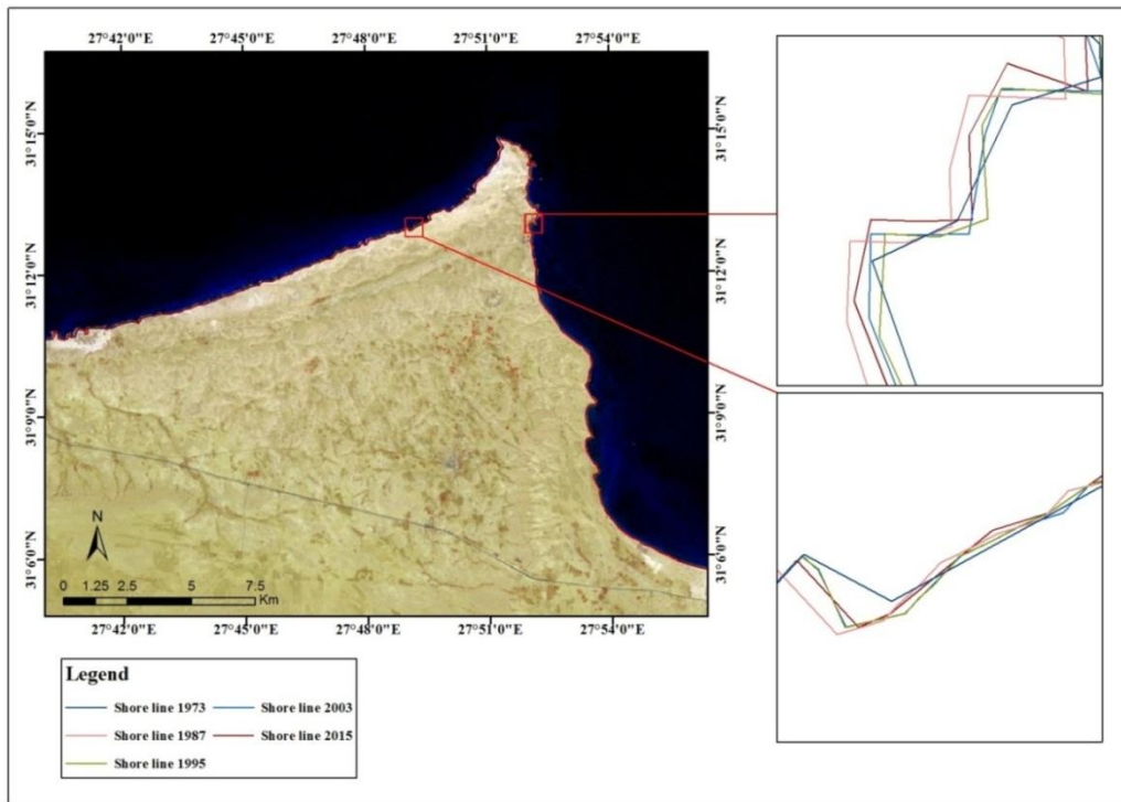
Fig. 4. Extracted Shoreline in different periods
