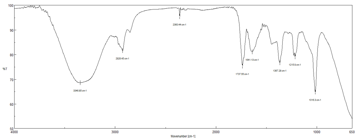
Fig. 2. Functional components in Passiflora edulis f. flavicarpaleaf
