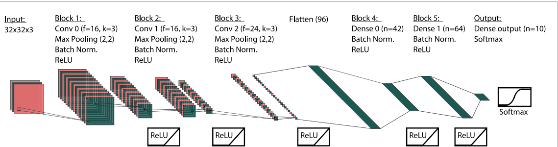
Figure 4. The neural network architecture, chosen through a Bayesian optimization over the hyperparameters, for classifying digits from the SVHN dataset. Each convolutional block consists of a convolutional layer, max pooling, batch normalization, and ReLU activation. The convolutional layers in the three convolutional blocks use 16, 16, and 24 filters, respectively, and each has a kernel size of 3 \times 3 . The pooling layers have a size of 2 \times 2 . The convolutional blocks are followed by two fully-connected layers consisting of 42 and 64 neurons, with batch normalization and ReLU activation. The bias term is removed from all layers except the final output layer.
