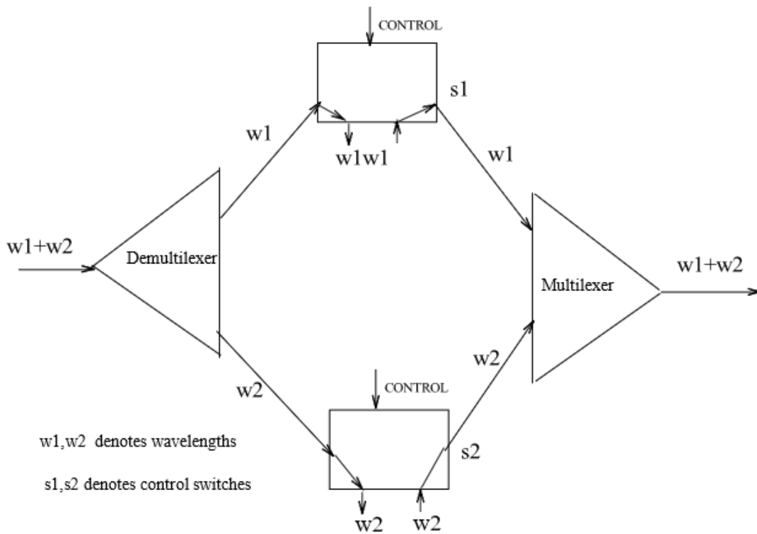
Fig. 10. A simple block diagram of wavelength add-drop multiplexer
