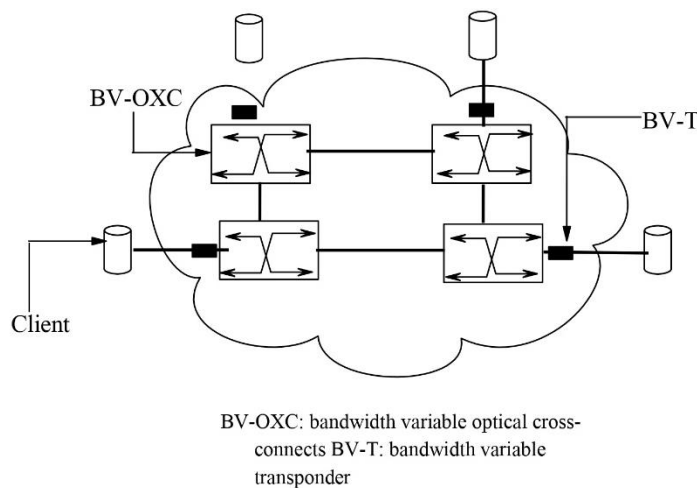
Fig. 13. A simple architecture of an elastic optical network system
