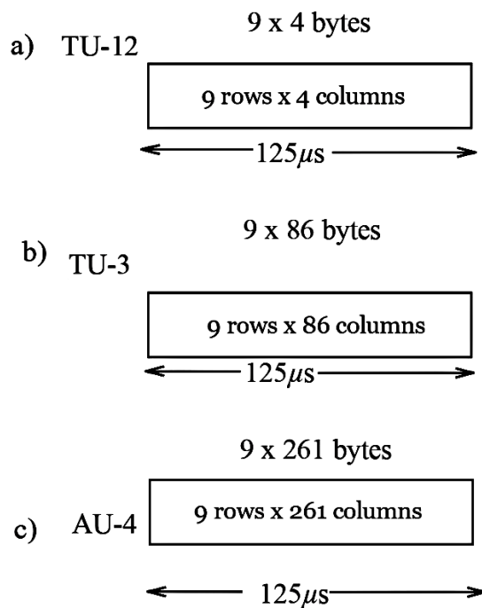
Fig. 8. Frame structure of different SDH multiplexing stages
