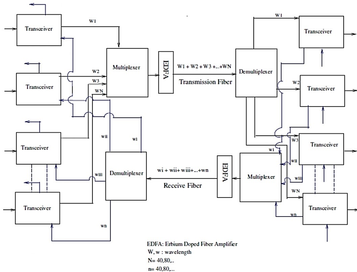
Fig. 9. A simple block diagram of a DWDM system
