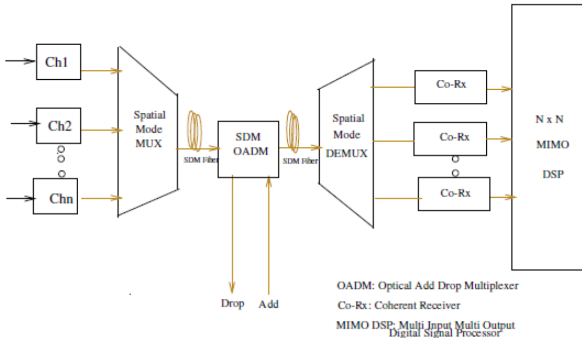
Fig. 17. SDM transmission system
