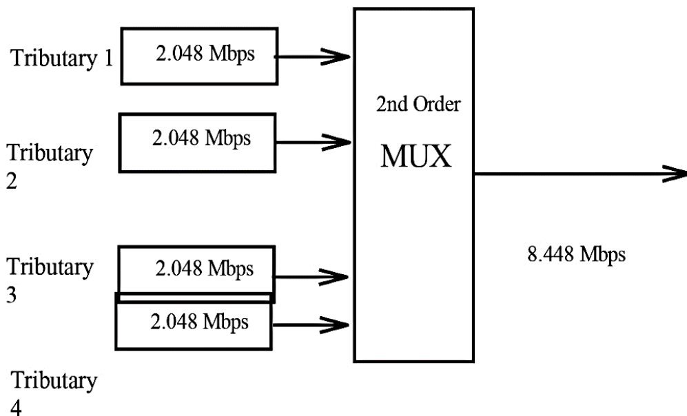
Fig. 3. Basic multiplexing method
