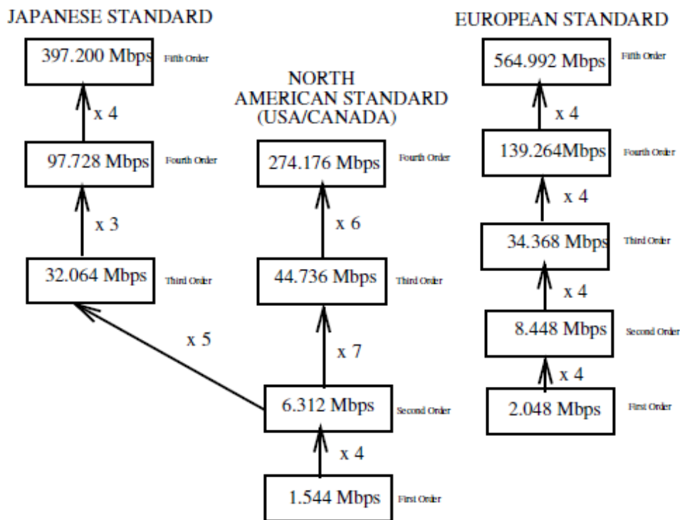
Fig. 2. Multiplexing tree for different PDH Hierarchies (American and Japan standards are the same for the first order and second order but differ in the higher orders)
