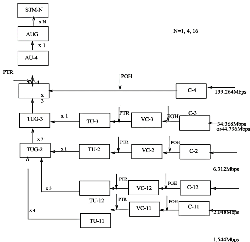
Fig. 5. Multiplexing tree for SDH
