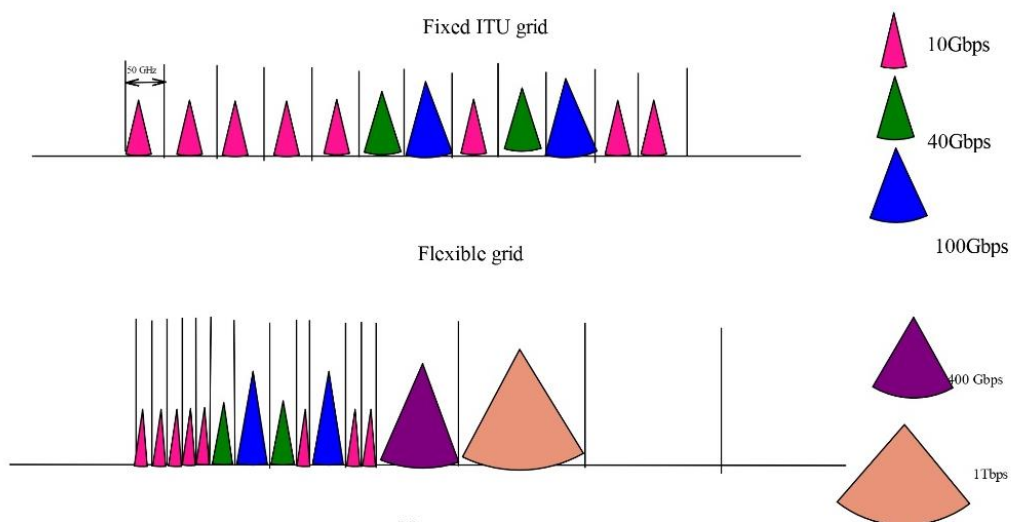
Fig. 12. Comparison of spectral widths in fixed and flexible grid optical networks
