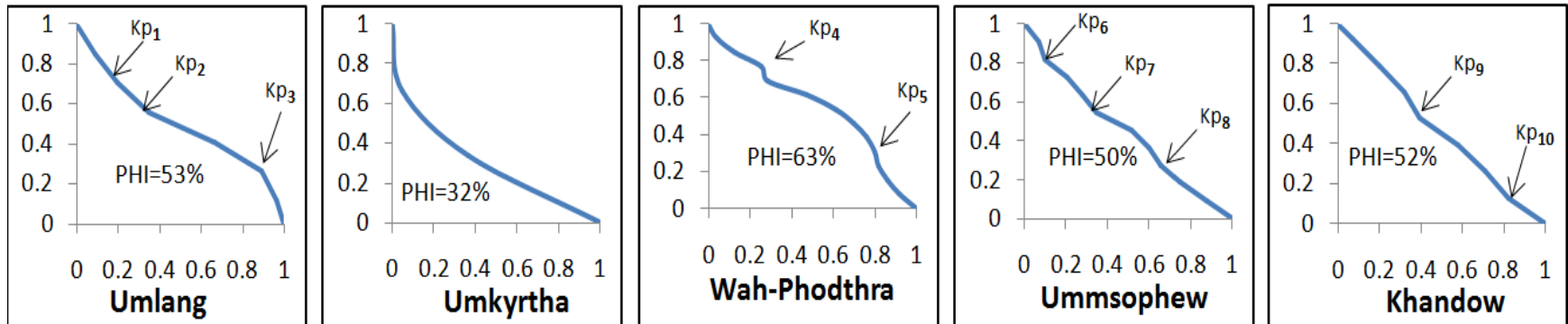
Fig. 5. Normalized longitudinal profiles
