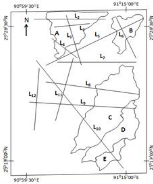
Fig. 7. Map showing distribution of major lineaments
