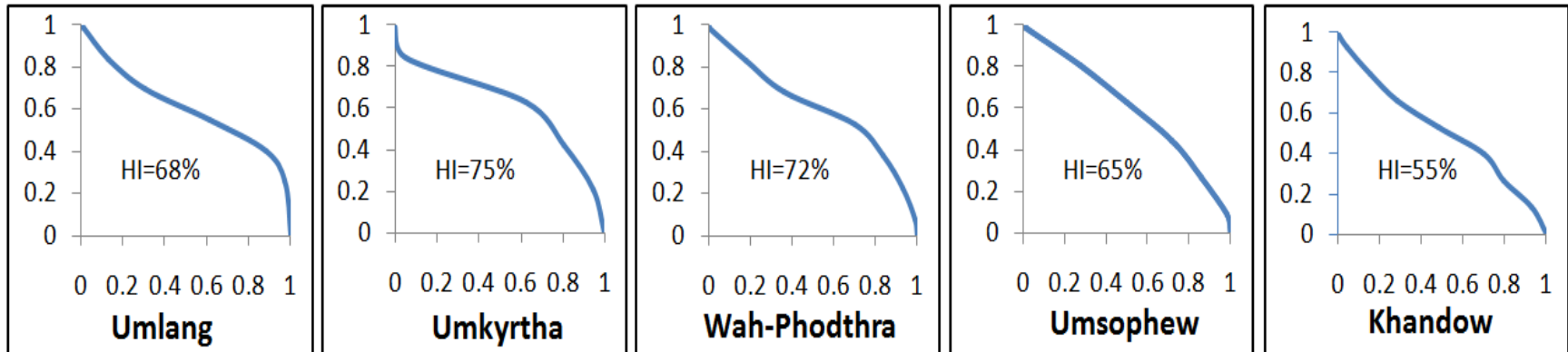
Fig. 4. Hypsometric curves of the sub-basins
