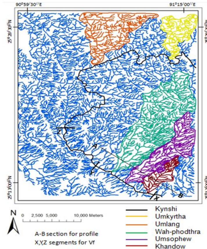
Fig.3. Drainage map of the study area
