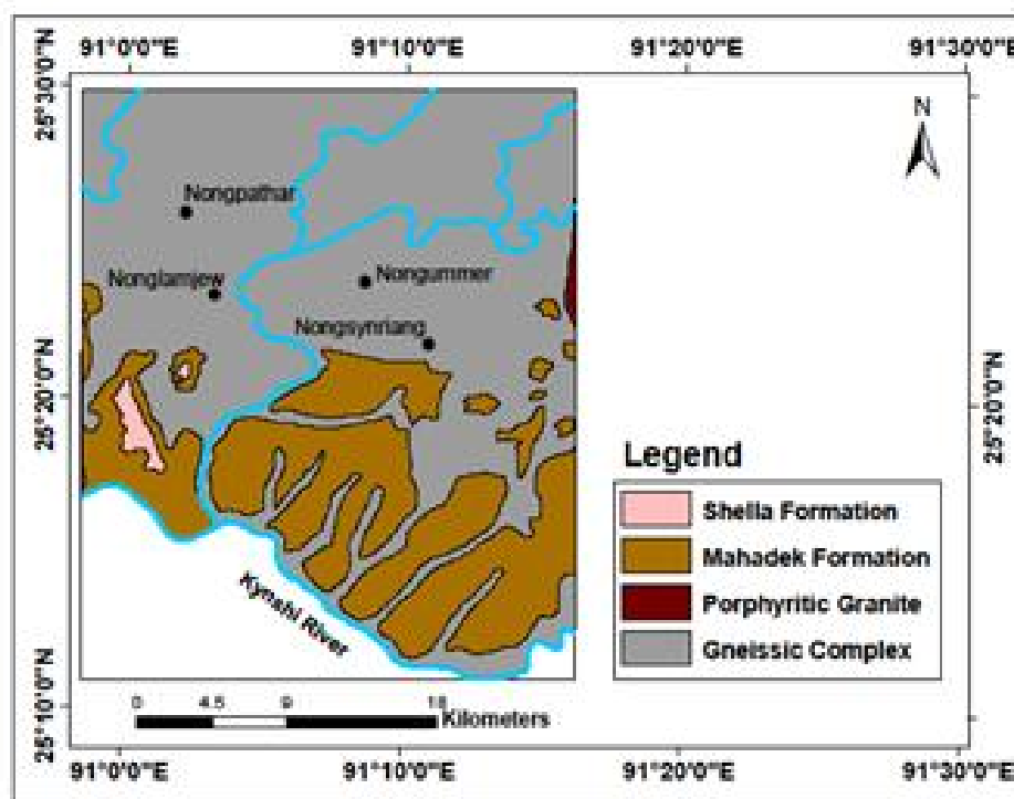
Fig. 2. Geological map of the study area - modified after Gangadharan [9]
