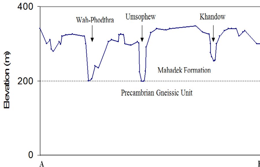
Fig. 6. Topographic profile along section A-B.
