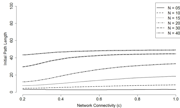
Figure 4: Path length of initial stable networks. For each network size ( N = 5, 10, 15, 20, 30 and 40 ) with each connectivity given from a range of values in continuous interval ( [0.2, 1] , step size 0.02 ), the path length (minimum time steps for reaching the equilibrium state) was tested based on an initial 10,000 randomly-generated stable gene regulatory networks. The system level parameters are set to be a = 100 , devT = 100 and \tau = 10 . Shaded areas represent 95\% confidence intervals based on 100 independent runs.
