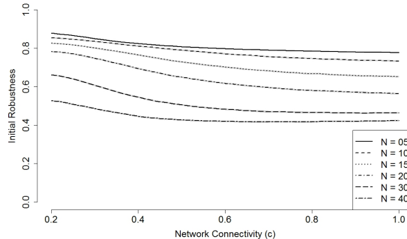
Figure 3: Robustness of initial stable networks. For each network size ( N = 5, 10, 15, 20, 30 and 40 ) with each connectivity given from a range of values in continuous interval ([0.2, 1], \text{step size } 0.02) , the robustness (proportion of stable networks after exposure to a single round of mutation) was tested based on an initial 10,000 randomly-generated stable gene regulatory networks. The system level parameters are set to be a = 100 , devT = 100 and \tau = 10 . Shaded areas represent 95% confidence intervals based on 100 independent runs.
