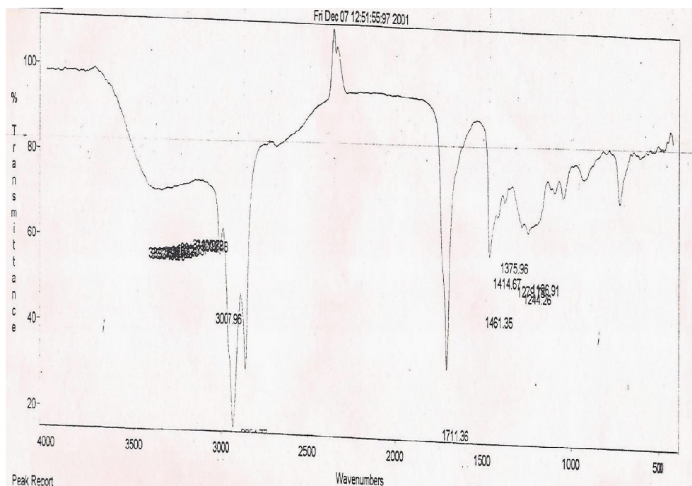
Fig. 1. Infrared spectrum of oil extract from Monodora myristica seeds
