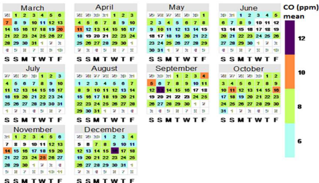
Fig. 4(a). Calendar plot for CO concentration in 2009 with a user-defined categorical scale
