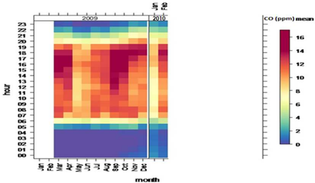
Fig. 3. Trend level plot function of CO concentration
