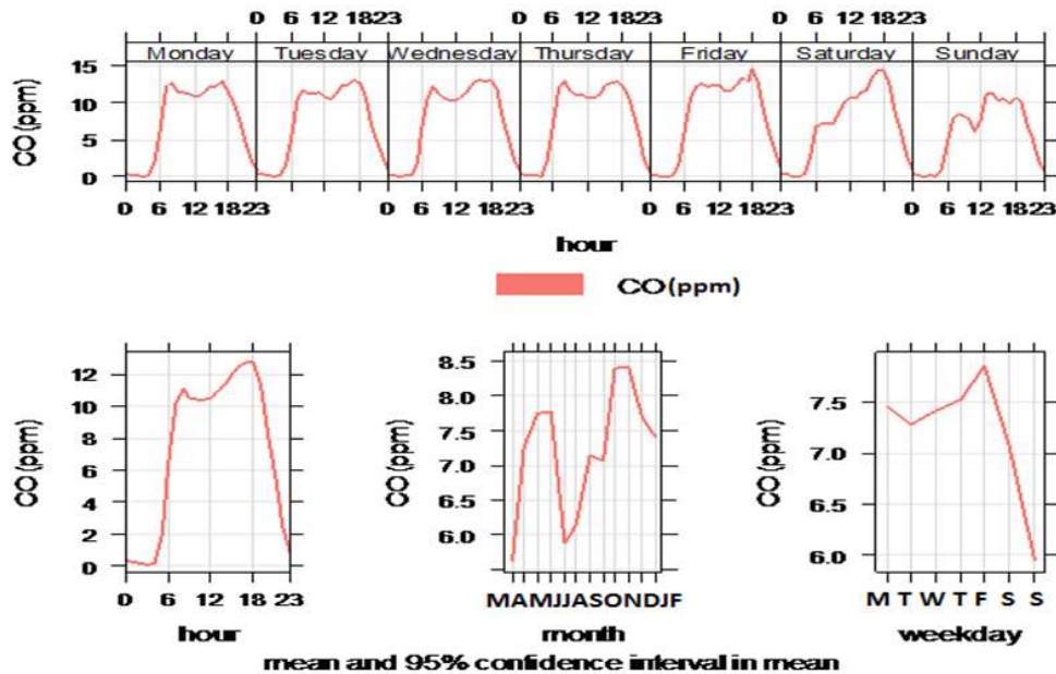
Fig. 2. Time variation function of CO concentration
