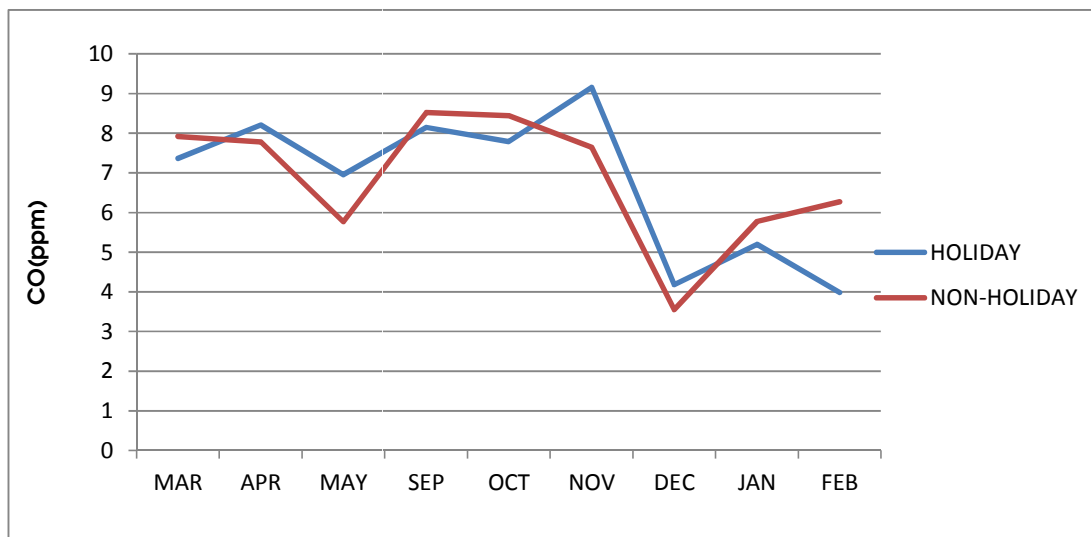
Fig. 7. Mean annual variation of CO concentration between the holiday and non -holiday effect
