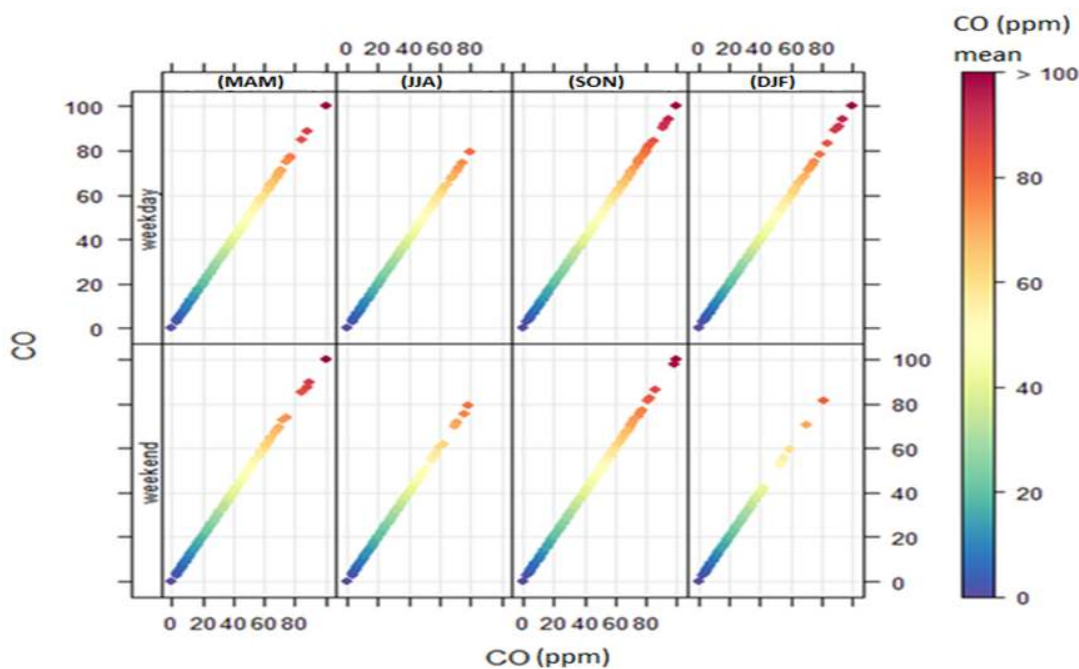
Fig. 5. Comparison between weekdays and weekends CO concentration for 15 minutes exposure by different level split by season
