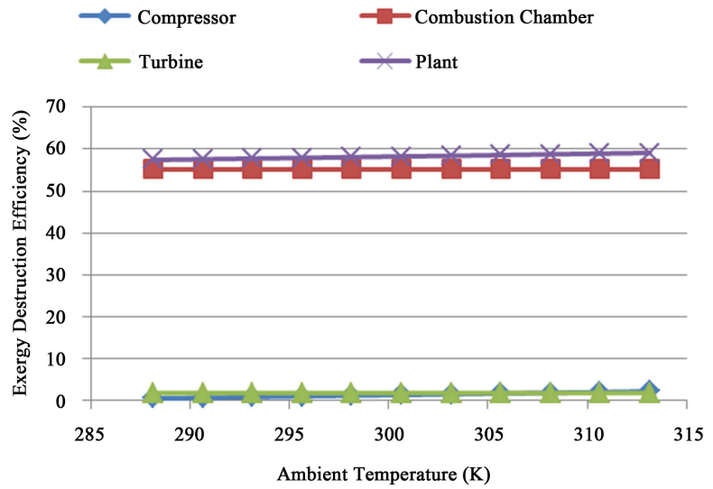
Figure 5. Change of exergy destruction efficiency with ambient temperature.
