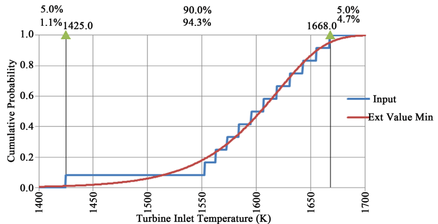
Figure 12. Ext value min distribution of temperature inlet temperature.
