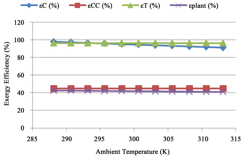
Figure 4. Change of exergy efficiency with ambient temperature.
