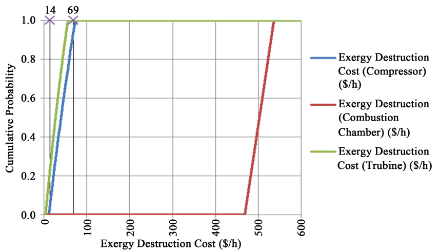
Figure 11. Cumulative probability density of exergy destruction cost with Ambient Scenario.
