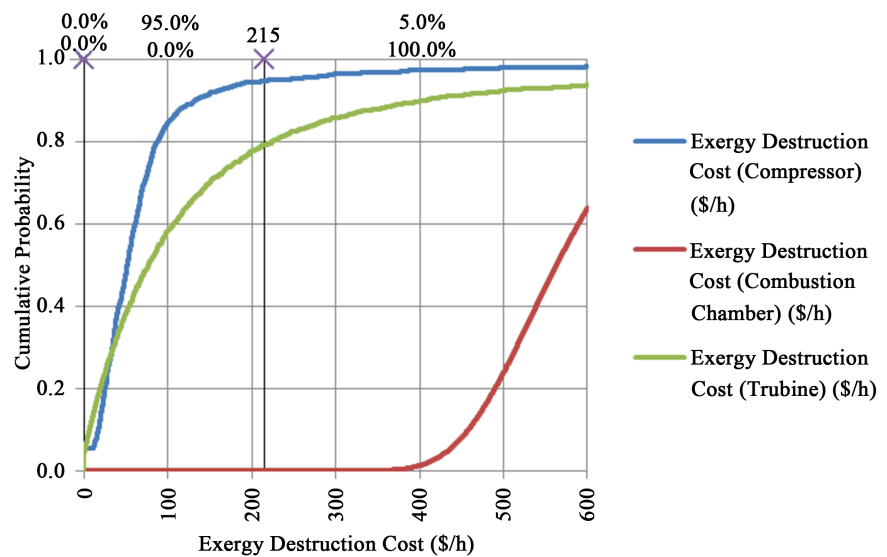
Figure 13. Cumulative probability density of exergy destruction cost.
