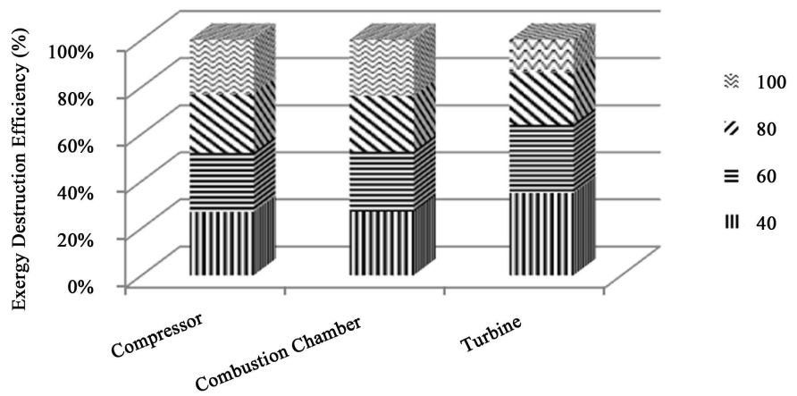
Figure 8. Percentage variation of exergy destruction with four part loads of 100 MW.
