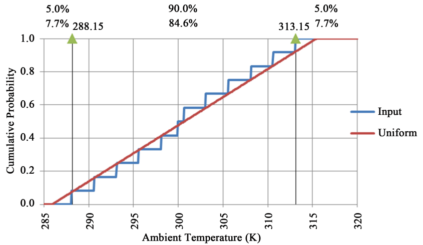
Figure 9. Uniform distribution of ambient temperature.
