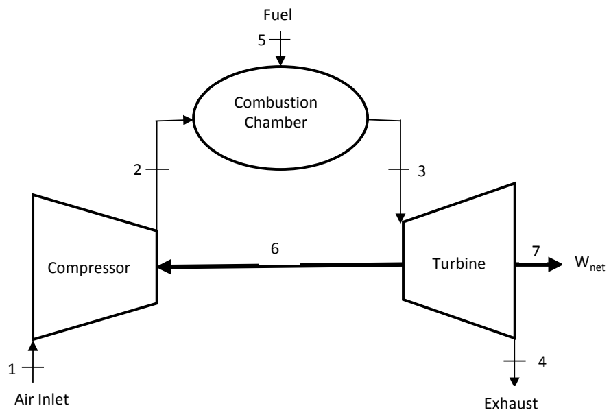
Figure 1. Schematic diagram of the gas power plant.
