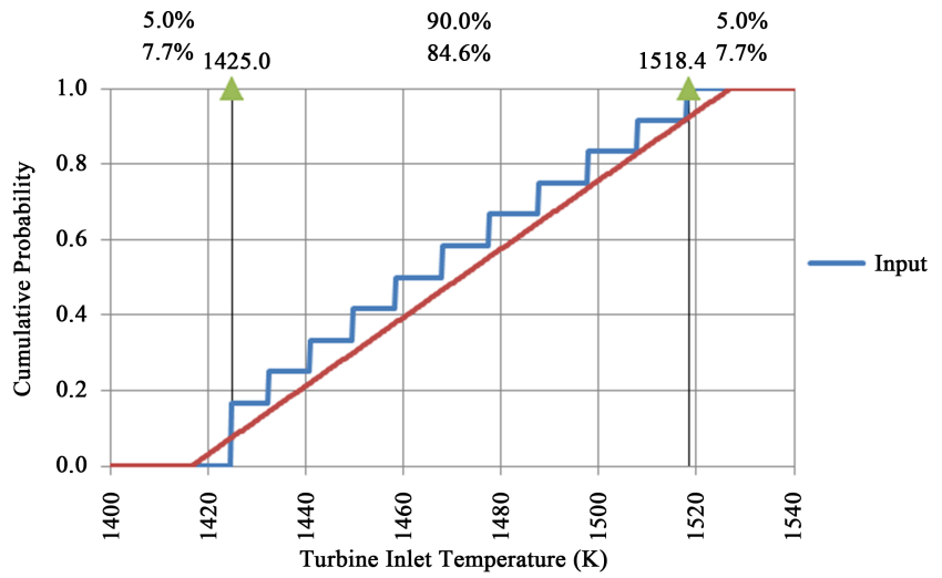
Figure 10. Uniform distribution of temperature inlet temperature.
