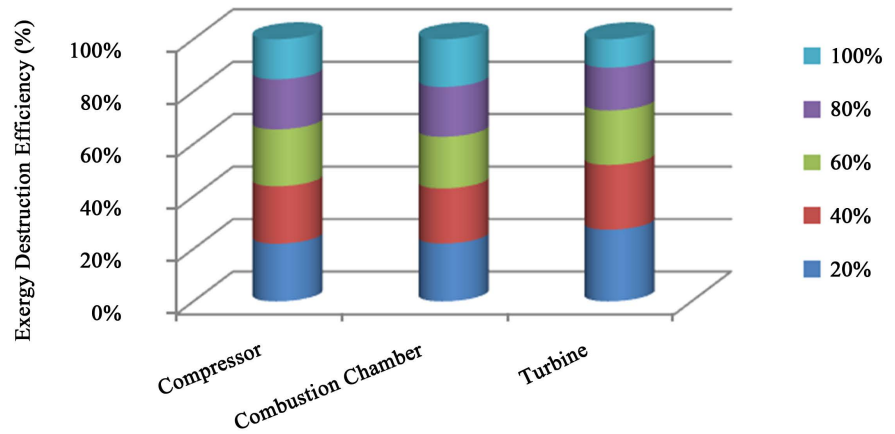
Figure 7. Percentage variation of exergy destruction with five part loads of 25 MW.
