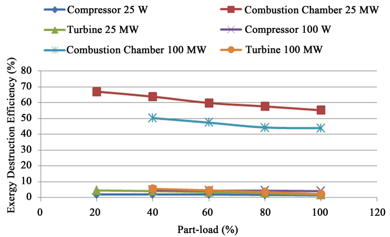
Figure 6. Exergy destruction efficiency with part-loads of 25 MW and 100 MW.
