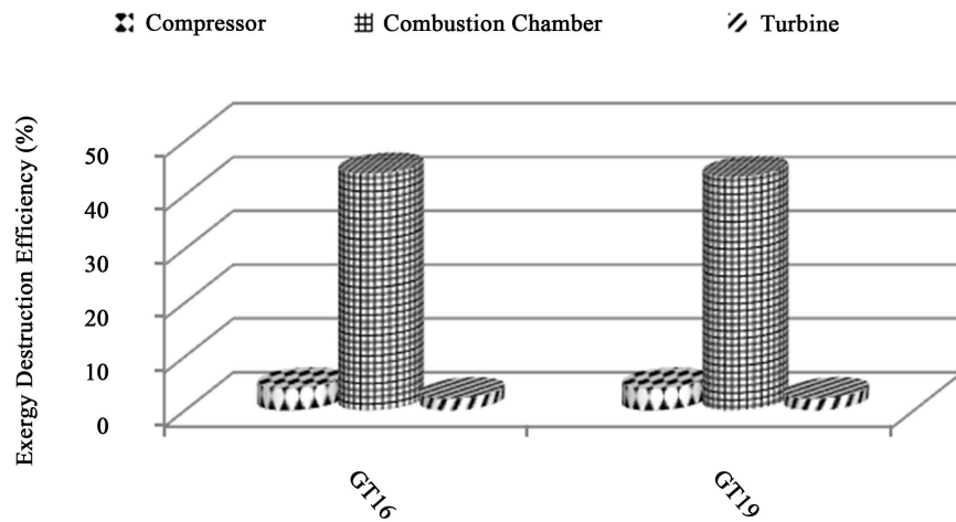
Figure 3. Exergy destruction efficiency of components of each plant.
