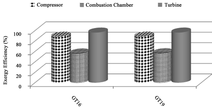
Figure 2. Exergy efficiency of components of each plant.
