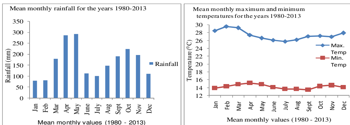
Fig. 1. Mean monthly rainfall and temperature data for the study sites from 1980-2013 (Source: [9])
